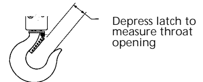
Figure 5 - Hook Inspection
