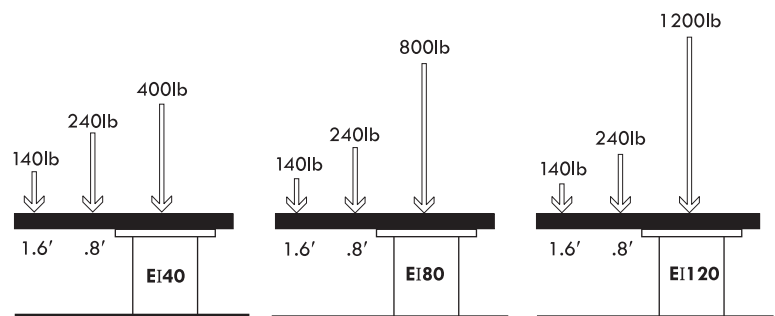
Dynamic Load Capacity
