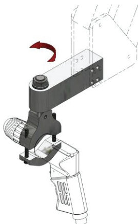
PISTOL GRIP V-BLOCK P/N: 658581
